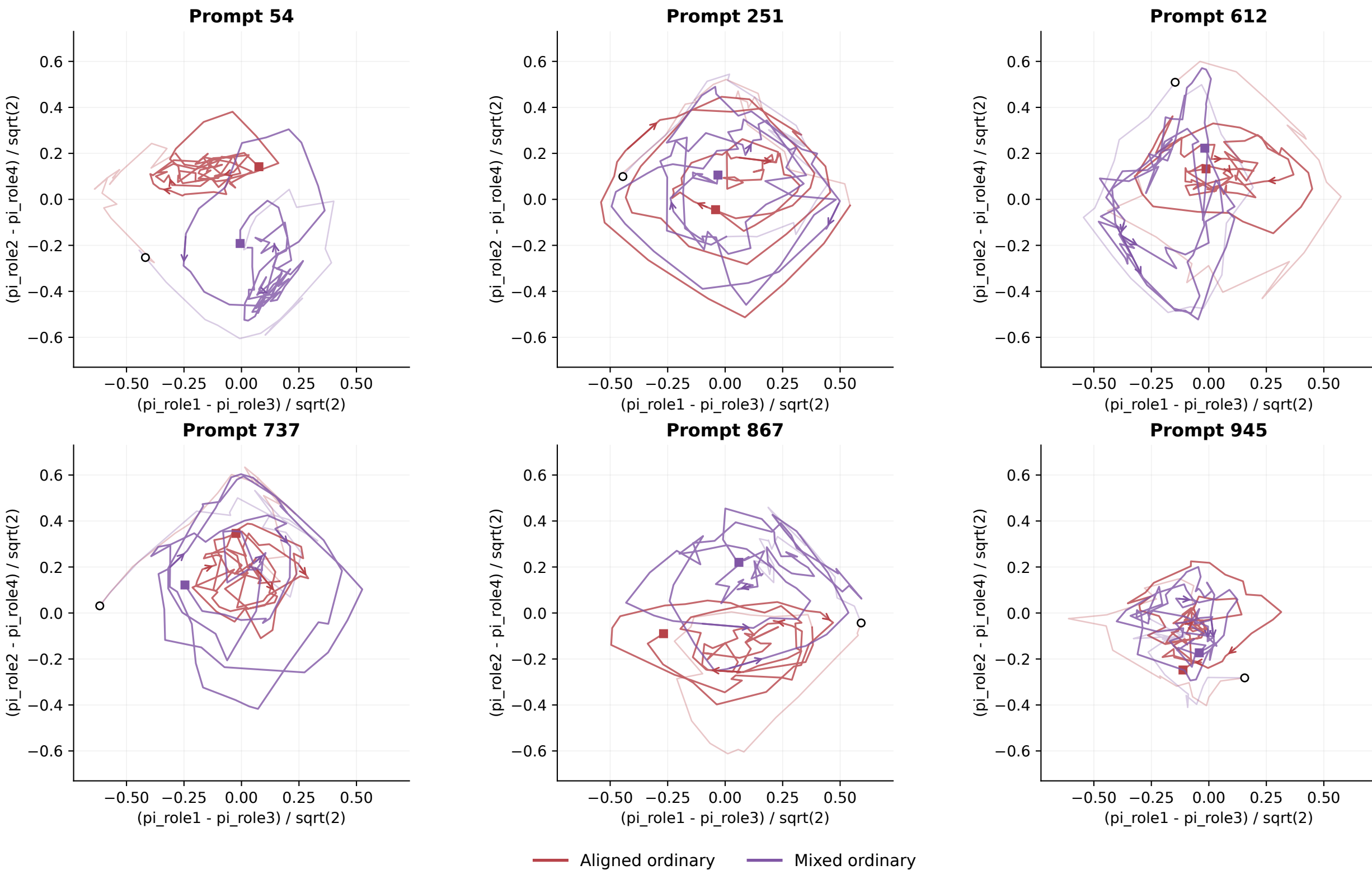
DPO | measured trajectories in a COMMON probability plane Fixed role contrasts, NOT an eigenmode or fixed-point error; circle=start, square=end; pale=0-20
