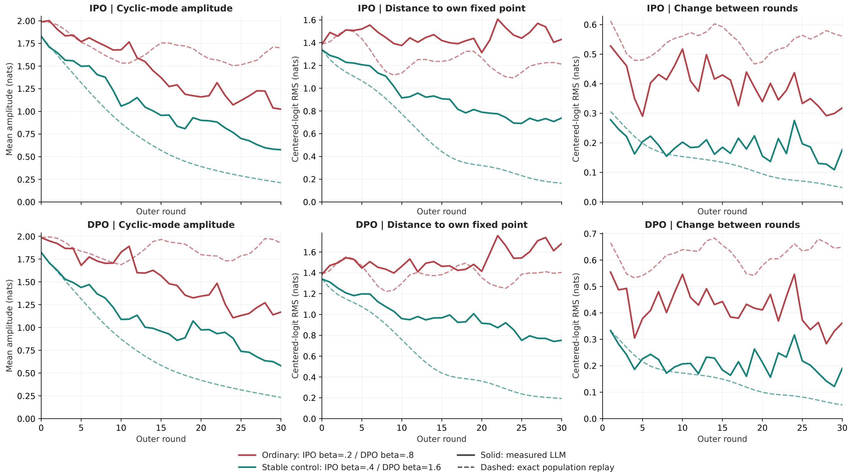
Stage A: measured LLM trajectories versus the calibrated population map 6 selected prompts, one seed; fixed points differ between beta controls
