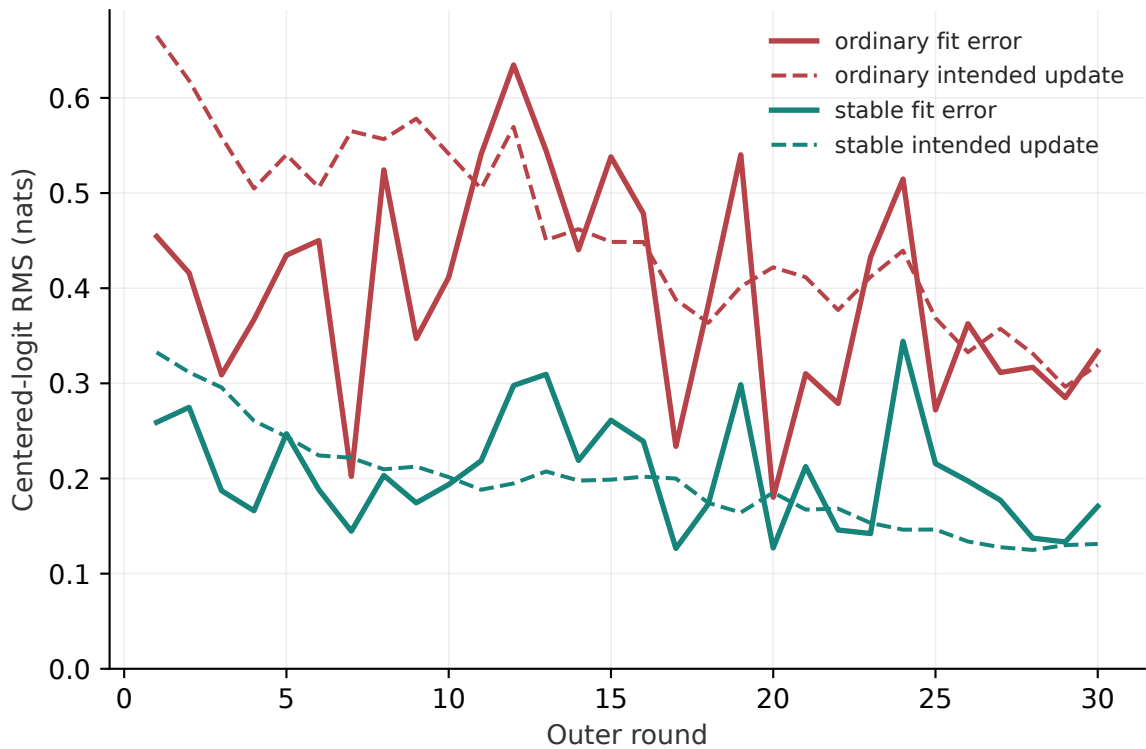
Inner-fit error is not negligible relative to the intended outer update
