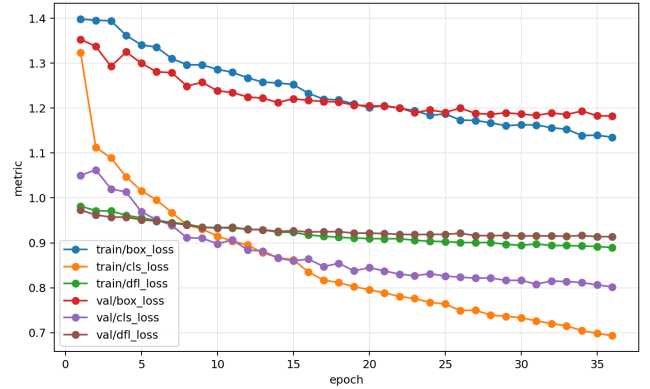
Figure 14: YOLO11m validation metrics and losses on VisDrone. The manually truncated run still achieved the best recorded score at epoch 36, while the losses were still decreasing slowly, suggesting possible remaining improvement with more epochs.
