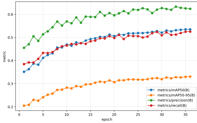
Figure 6: YOLO11m validation metrics on VisDrone. The manually truncated run still achieved the best recorded score at epoch 36.
