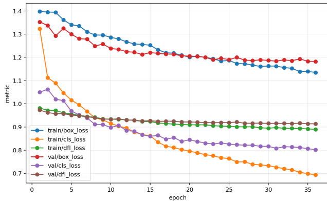
Figure 7: YOLO11m training and validation losses. The losses were still decreasing slowly, suggesting possible remaining improvement with more epochs.
