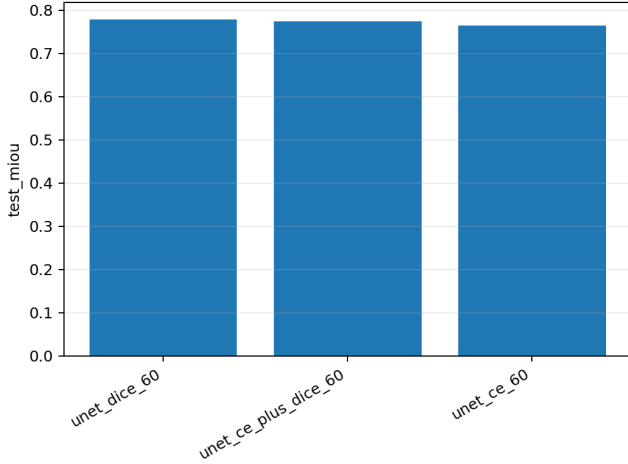
Figure 4: Test mIoU for the required 60-epoch segmentation losses. Dice loss gives the strongest required result.
