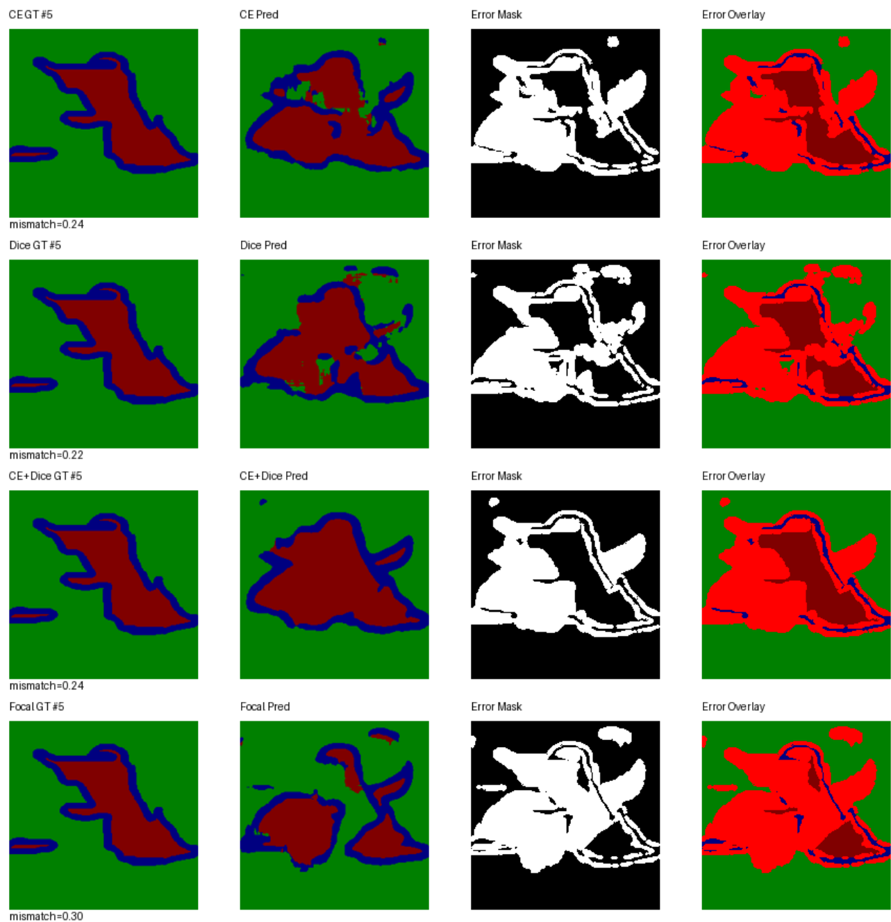
Figure 5: Segmentation failure cases. The most persistent errors occur at object boundaries, thin structures, and low-contrast regions rather than in the coarse pet/background separation.
