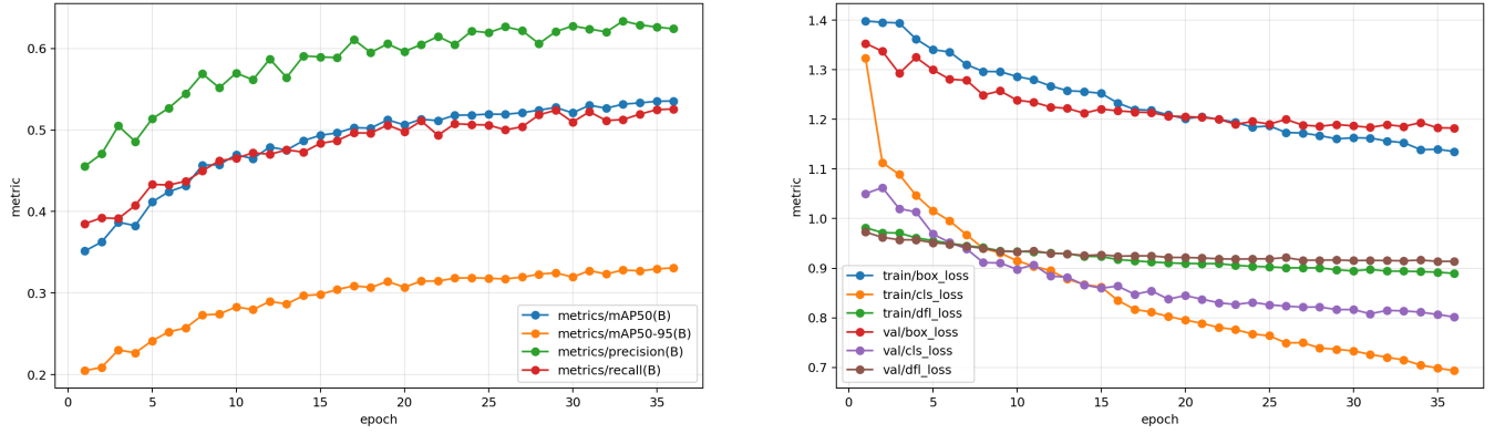
Figure 15: YOLO11m validation metrics and losses on VisDrone. The manually truncated run still achieved the best recorded score at epoch 36, while the losses were still decreasing slowly, suggesting possible remaining improvement with more epochs.
