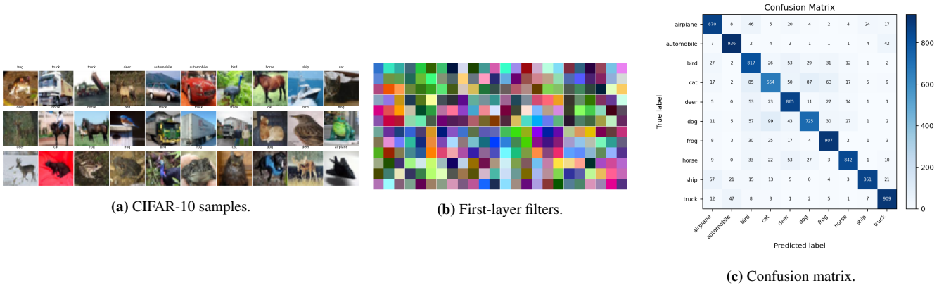
Figure 3: Interpretation artifacts generated from the final VGG-A-BN-GELU checkpoint.
