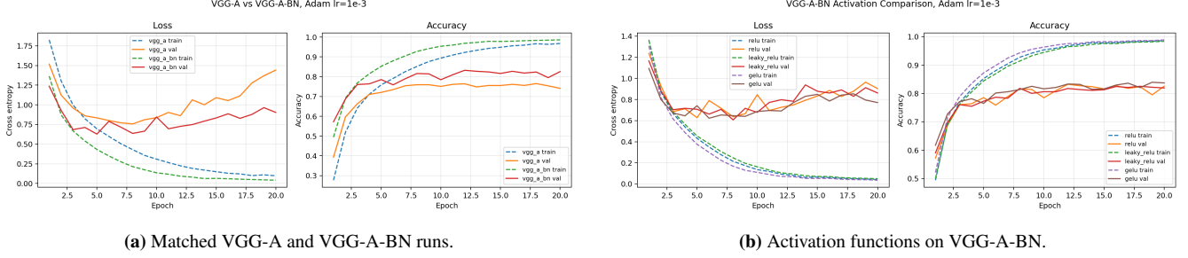
Figure 1: Training curves for the central BN comparison and the activation ablation.
