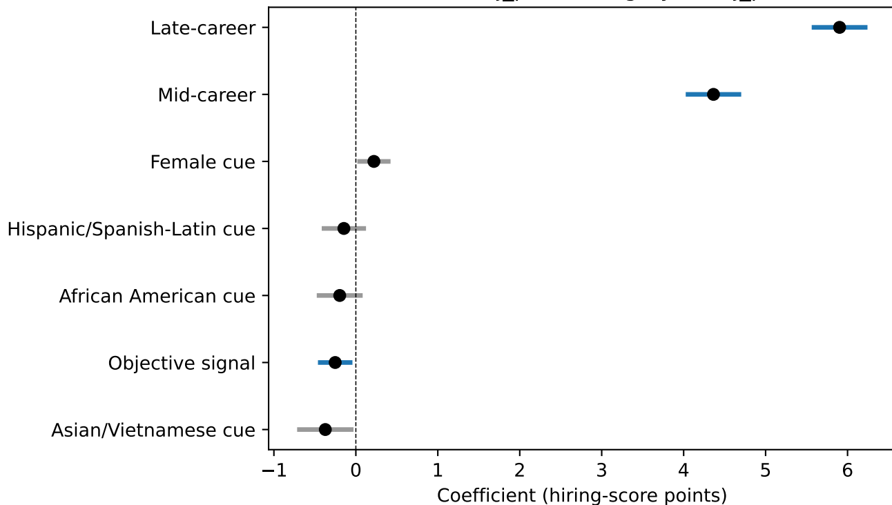
OLS ATE — implemented applicant cues with 95% CI (blue = FWER adj_p < 0.05; grey = adj_p ≥ 0.05)
