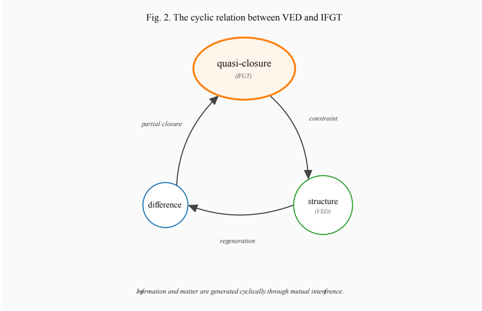
Figure 2: The cyclic relation between VED and IFGT. Informational and physical descriptions are coupled through mutual interference. The quasi-closure is positioned as the central mediating node.
