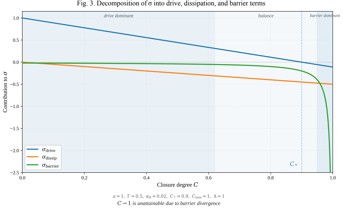
Figure 3: Decomposition of \sigma into drive, dissipation, and barrier terms. The barrier term diverges as C \rightarrow 1 , ensuring that complete closure is unattainable.
