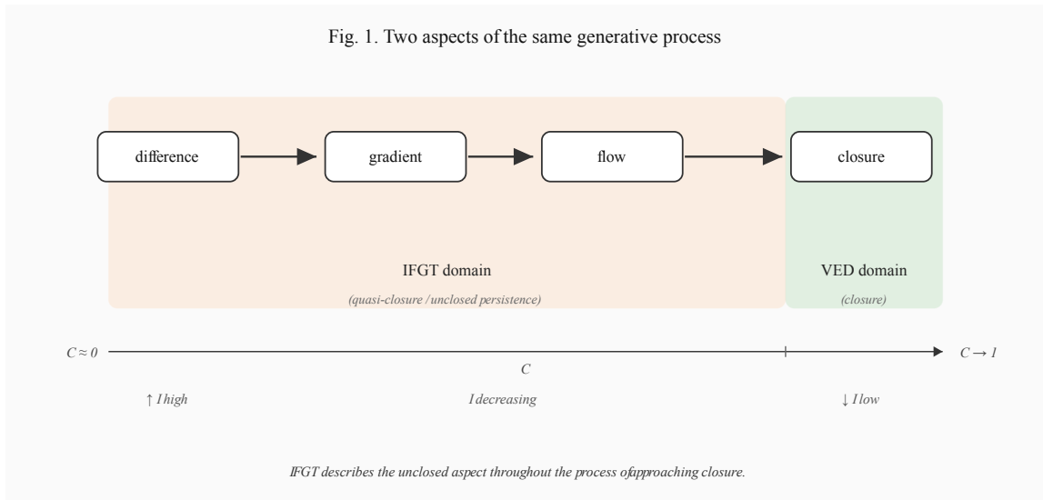
Figure 1: Two aspects of the same generative process. The VED chain (difference \rightarrow gradient \rightarrow flow \rightarrow closure) unfolds across the closure-degree axis C . IFGT covers the region where C has not yet reached unity; VED describes the fully closed region.
