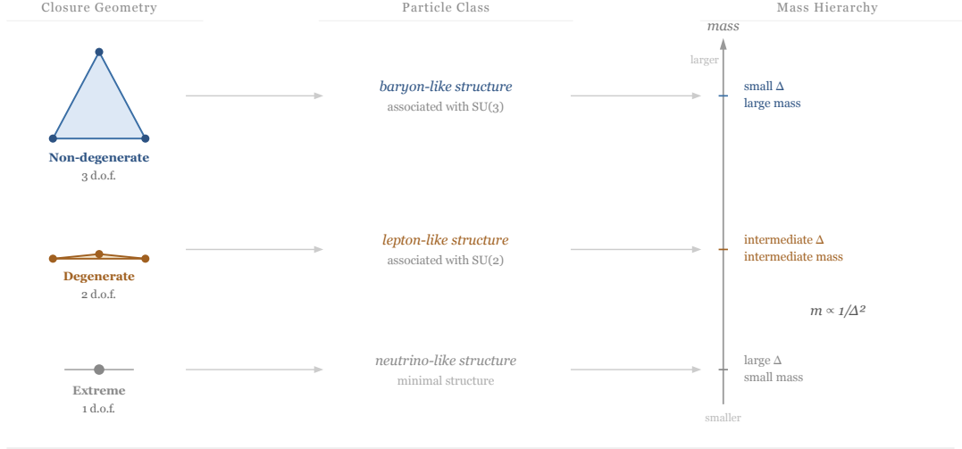
Figure 3: Particle classes as closure geometry. Triangular closure admits three structural regimes depending on degeneracy. These regimes correspond to baryon-like, lepton-like, and neutrino-like structures. Mass is associated with the distance from complete closure, with m \propto 1/\Delta^2 .
