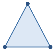
Non-degenerate 3 d.o.f.
