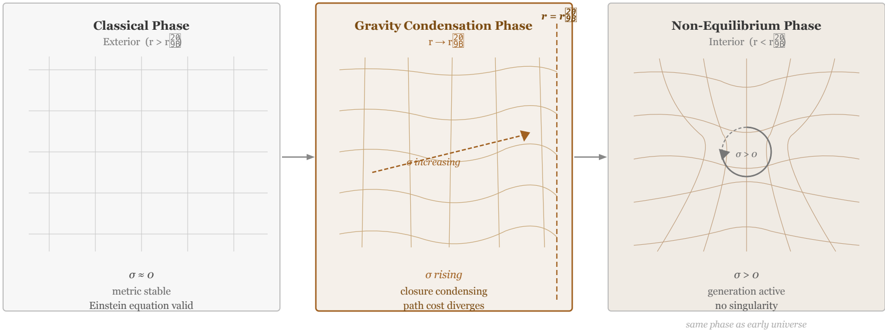
Figure 2. Phase transition across the horizon.
