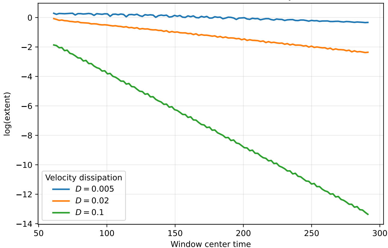
Finite-Window Phase Extent Decay
