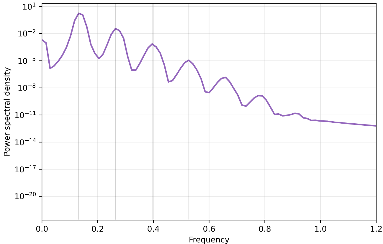
Spectrum of the Closure Velocity v(t)
