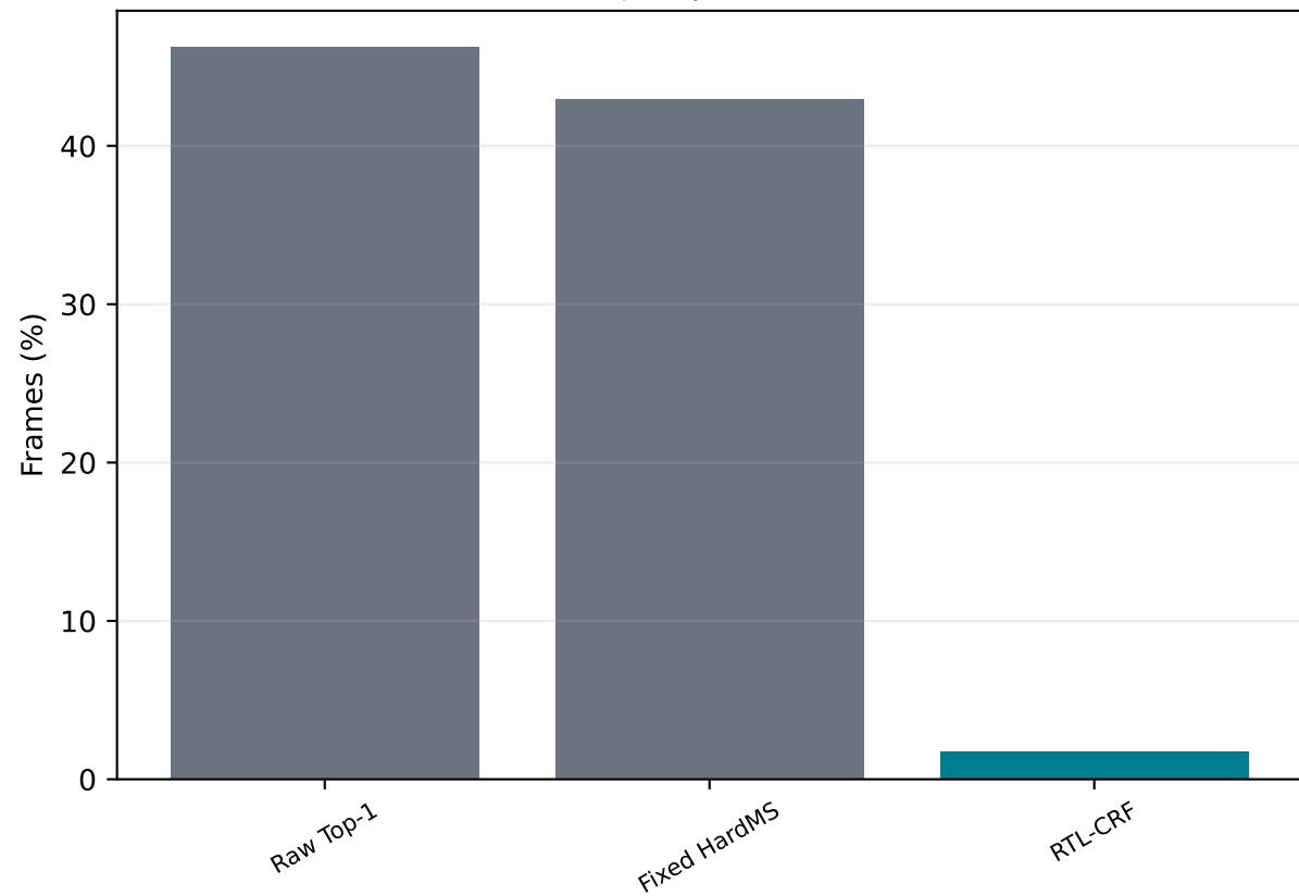
Jump rate
