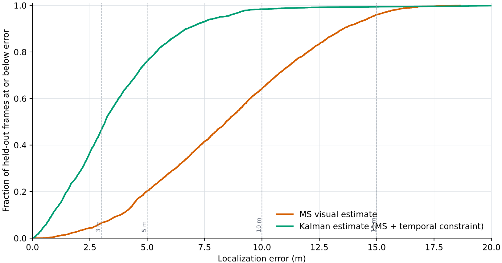
Cumulative localization-error distribution (Routes B + C)
