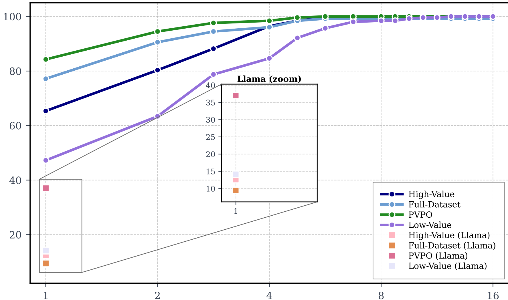
Stability (%), iid
