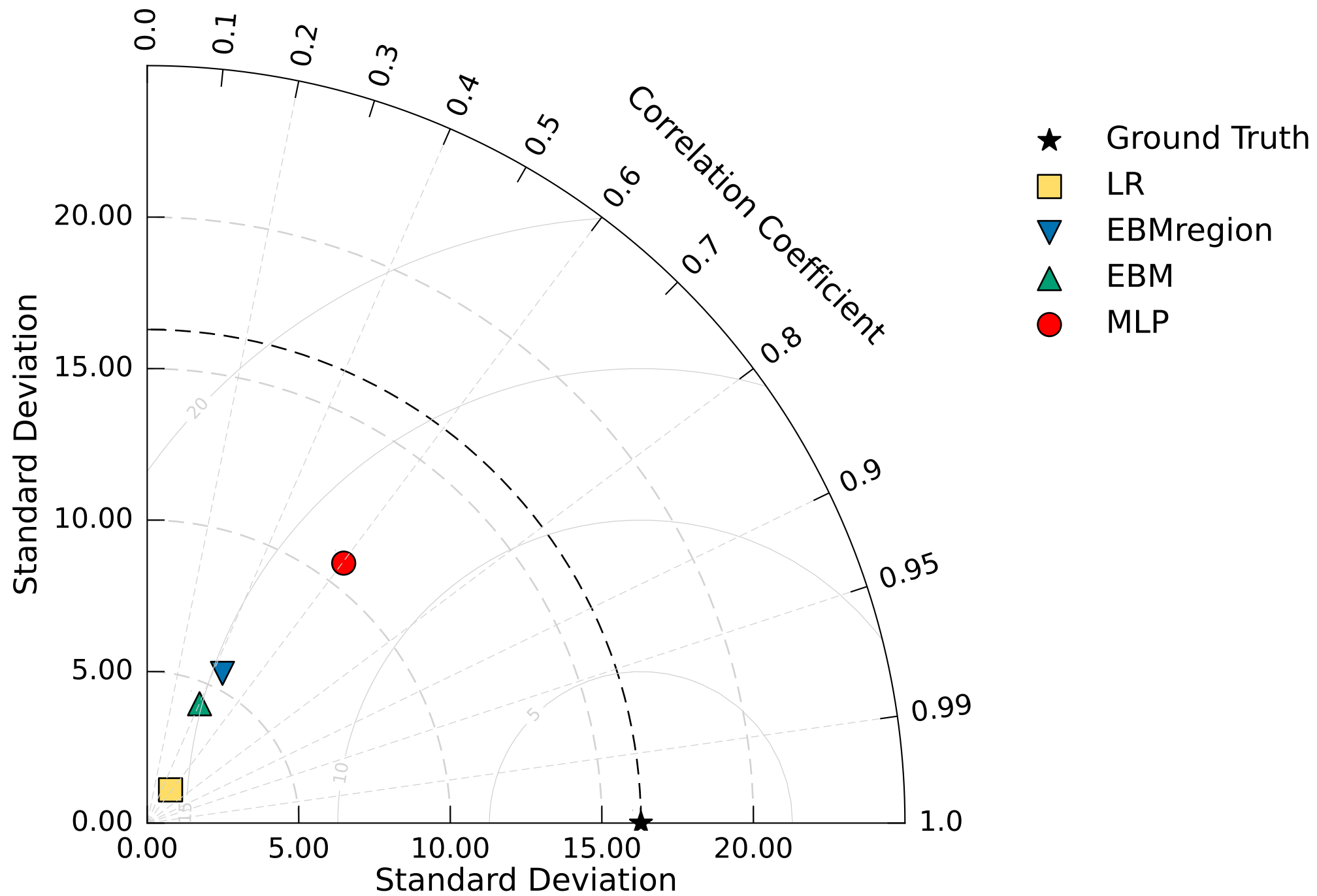
Taylor Diagram
