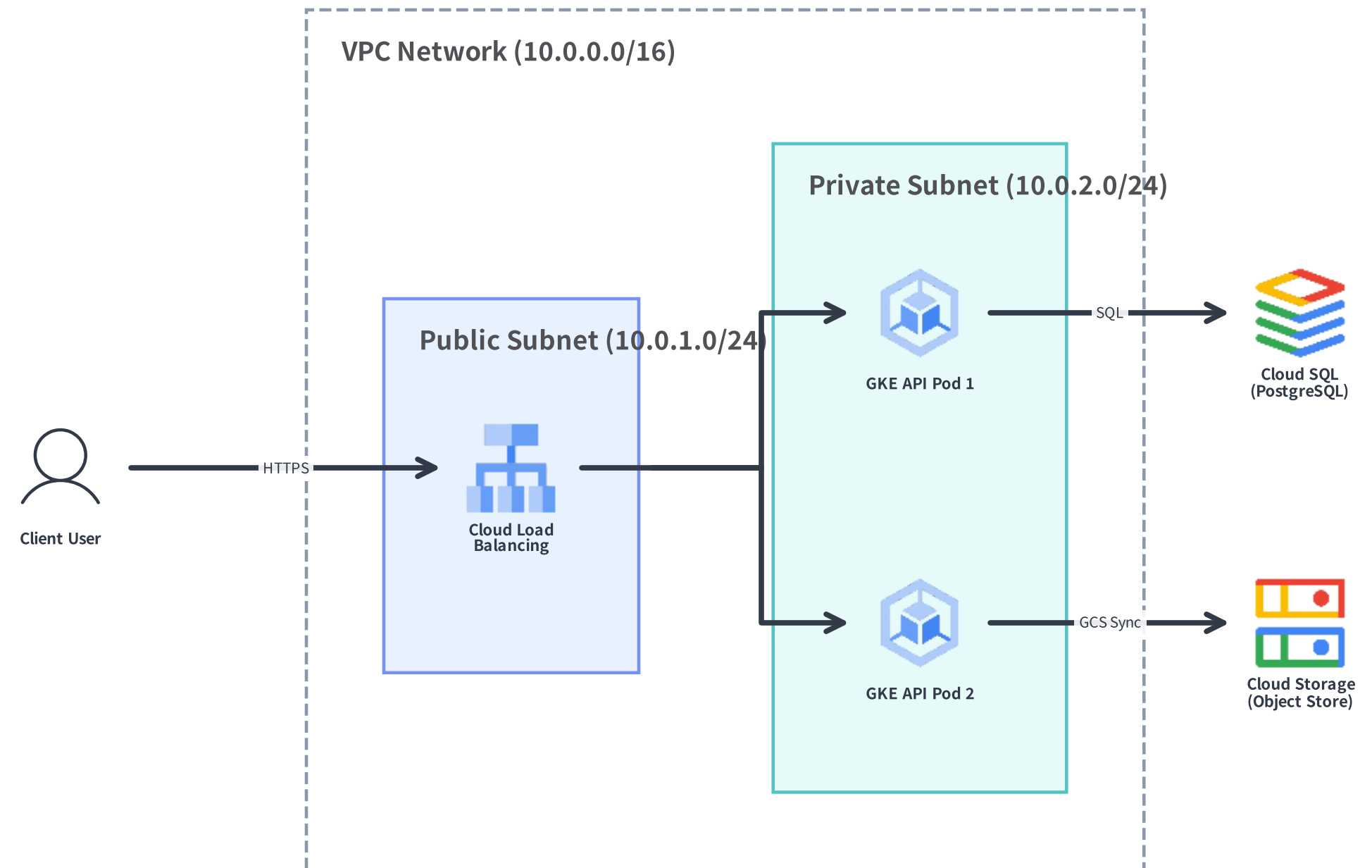
t Google Cloud VPC Architecture
