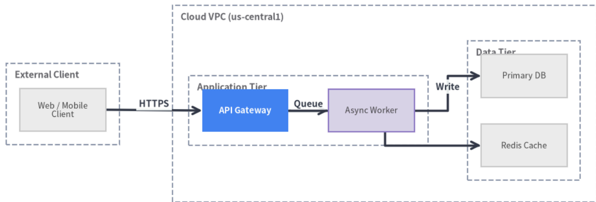
Figure 10.2: Auto-Layout and Cluster Packing with ArchitectureGraph
