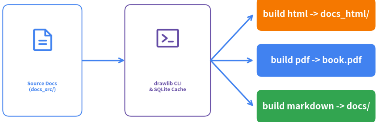
Figure 12.1: Unified Drawlib CLI Build & Preview Pipeline
