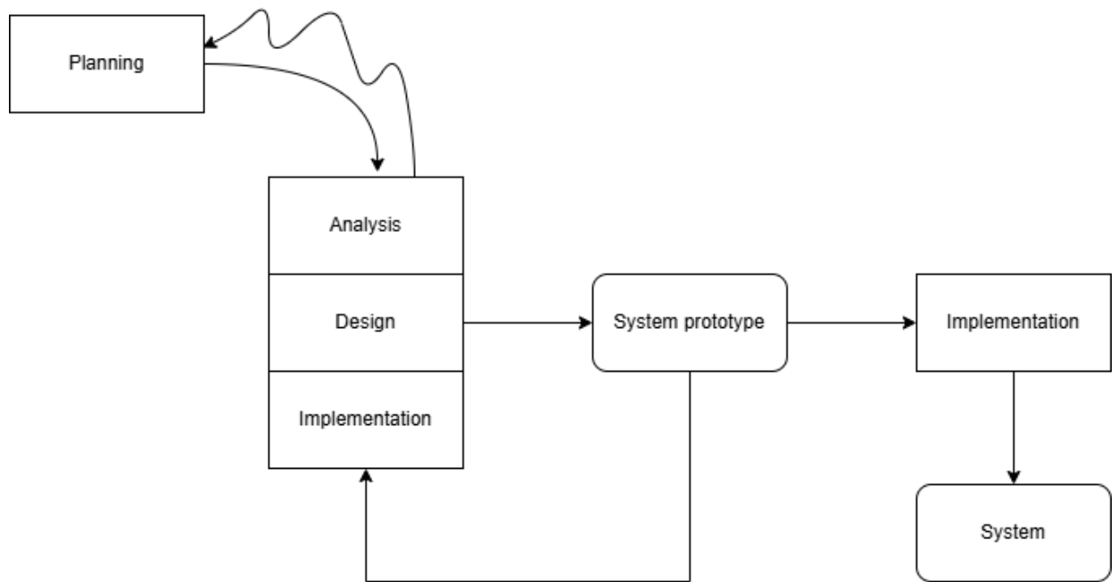
figure 3.4.1 Prototyping Methodology
