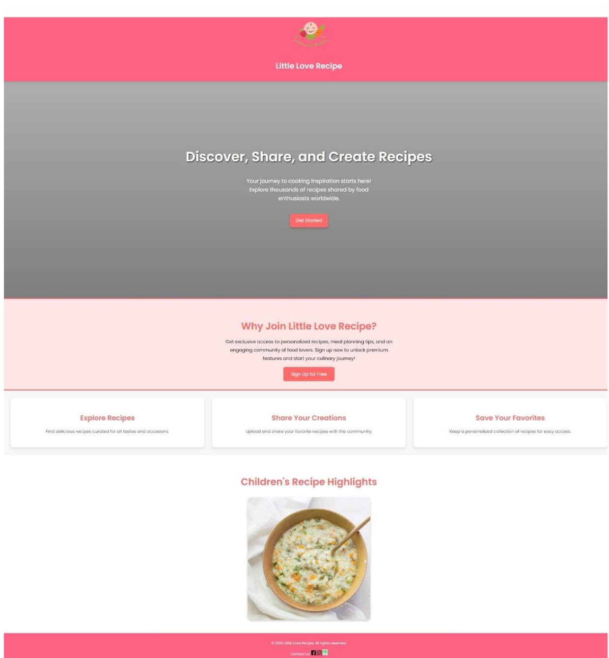
figure 3.3.0 Landing Page
