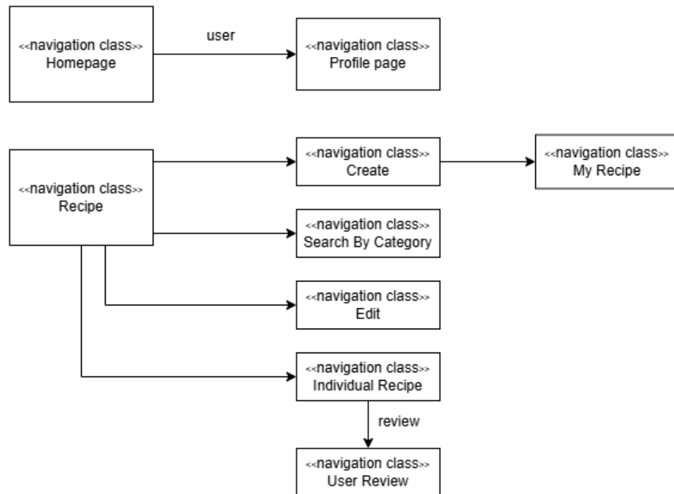
figure 3.2.1 Hypertext Navigation Modelling of Web-based Applications
