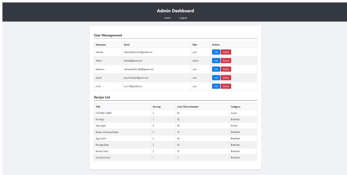
figure 3.3.13 Admin Dashboard
