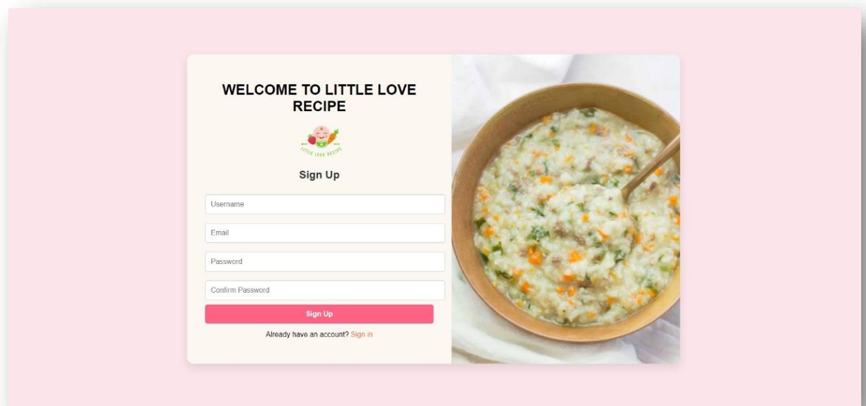
figure 3.3.1 Sign-up page
