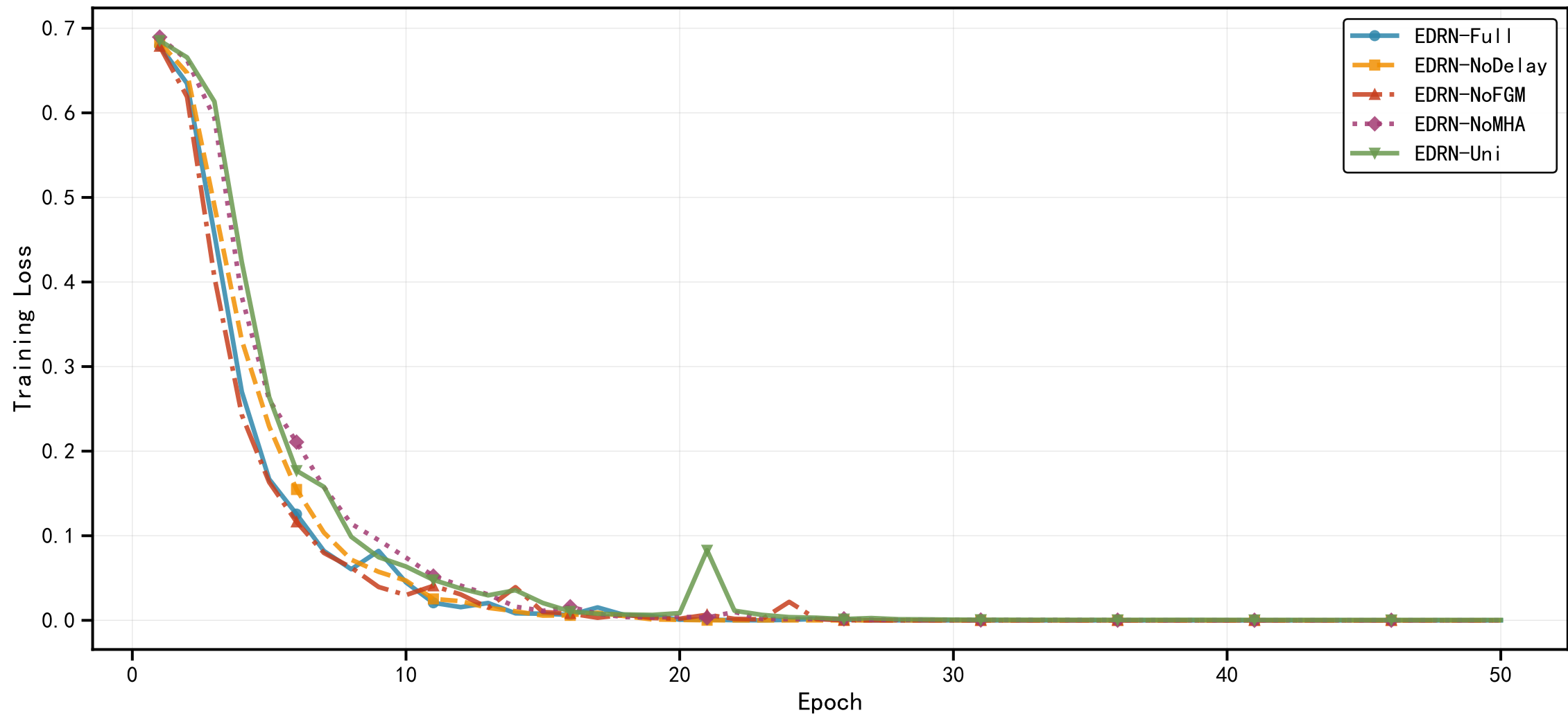
Figure 4: Ablation Study – Training Loss Curve (50 Epochs)
