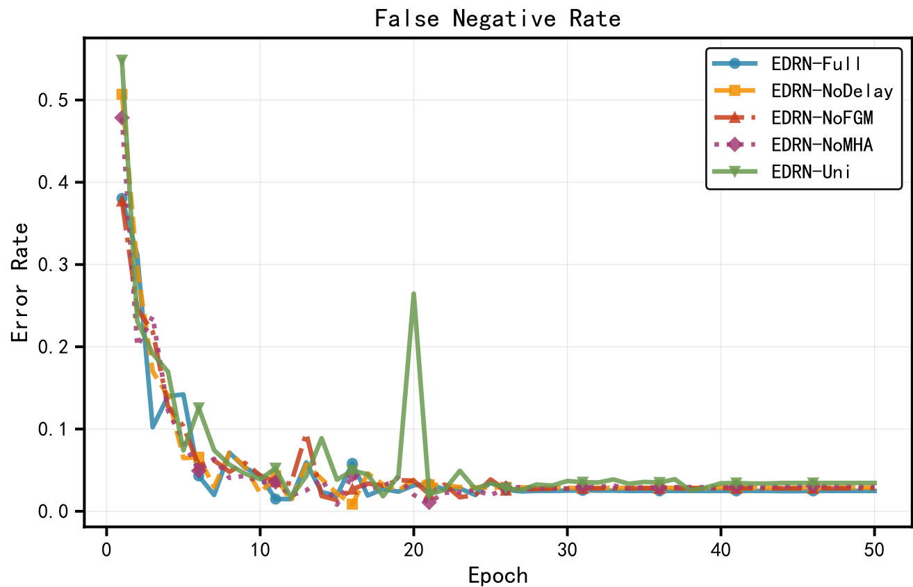
Figure 7: Ablation Study – FPR/FNR Evolution
