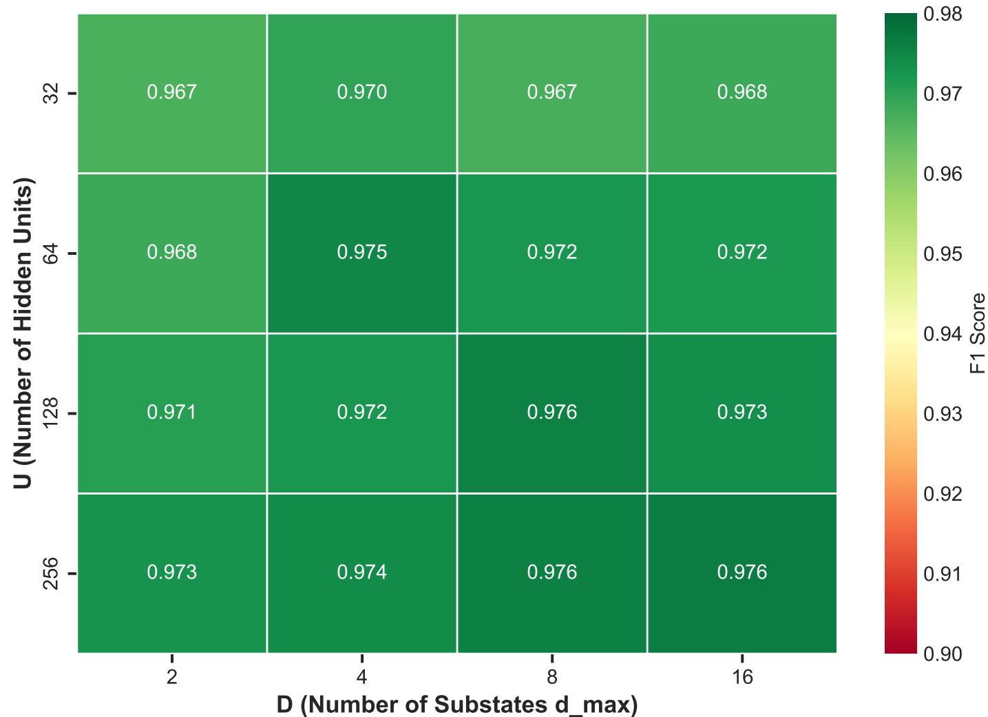
Figure 7: Hyperparameter Grid Search - F1 Score Heatmap
