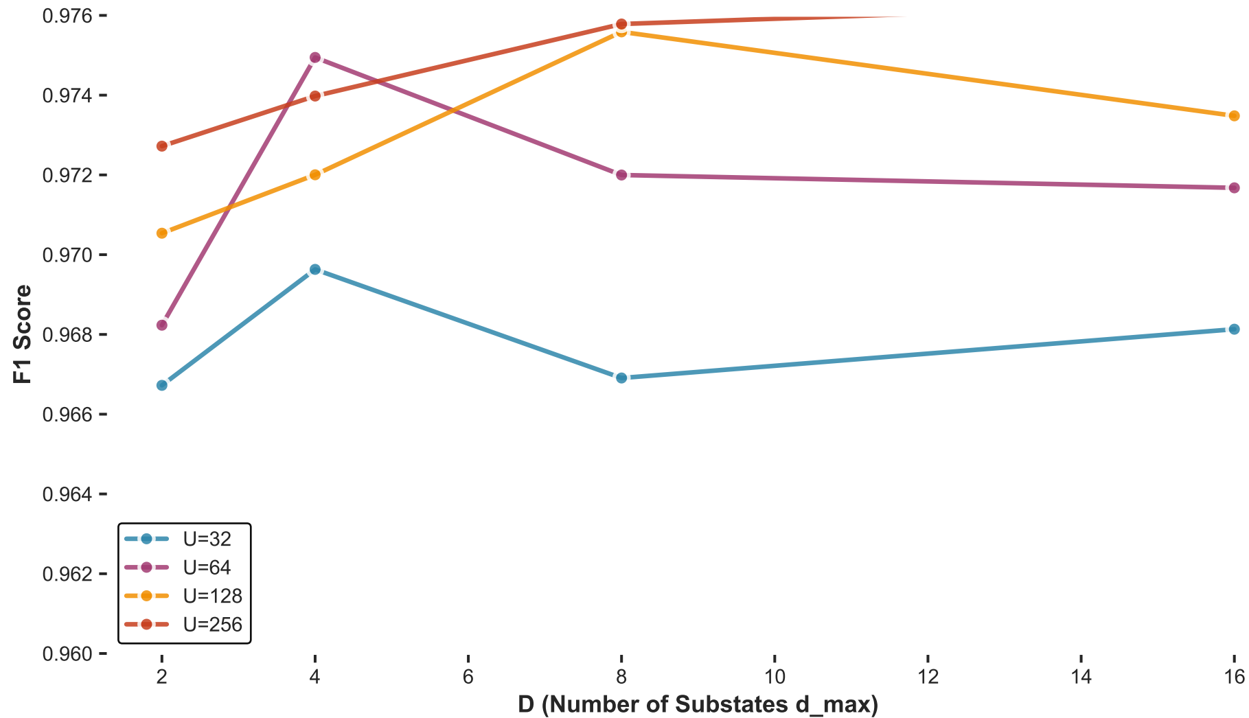
Figure 8: Hyperparameter Tuning - F1 Score Trend with D
