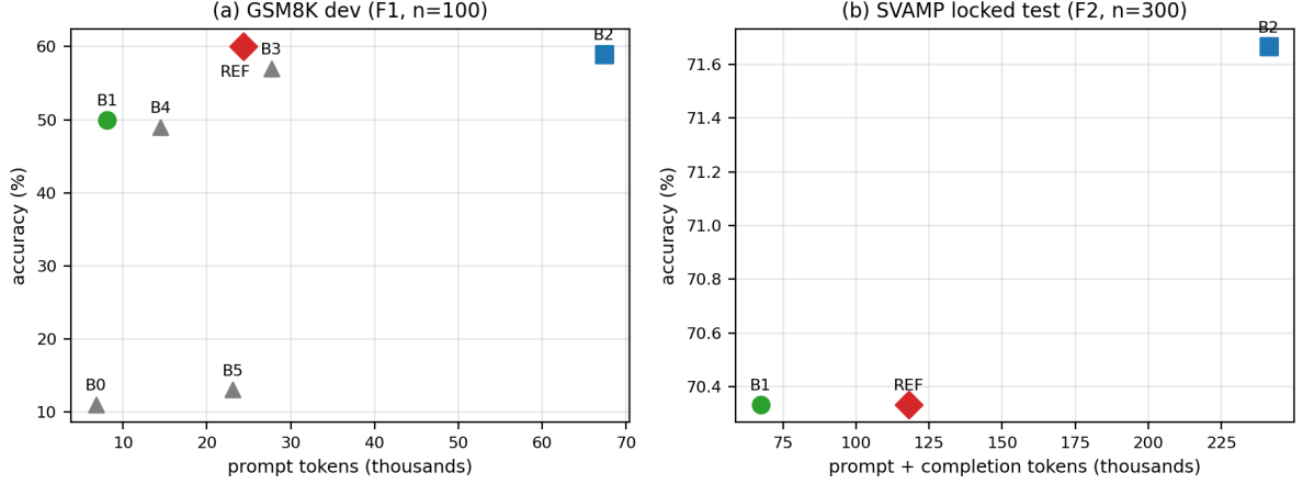
Figure 1: Accuracy vs. inference-token cost, separate panels per dataset. (a) GSM8K dev (F1, n=100 , prompt tokens): direct presets collapse; CoT presets cluster at 49–60% with \sim 8\times prompt-token spread; REF ties B2 at mid-range cost. (b) Locked SVAMP test (F2, n=300 , prompt+completion tokens): B1 attains REF’s observed accuracy at the lowest cost; B2 is nominally highest in both.
