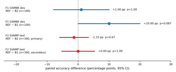
Figure 2: Paired accuracy differences with 95% bootstrap CIs (blue: F1 GSM8K dev; red: F2 locked SVAMP test). CIs are sampling uncertainty, not equivalence bounds: absence of a detectable difference does not establish that the compared configurations are equal.
