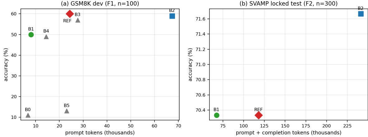
Figure 1: Accuracy vs. inference-token cost, separate panels per dataset. (a) GSM8K dev (F1, n=100 , prompt tokens): direct baselines collapse; CoT configurations cluster at 49–60% with \sim 8.3\times prompt-token spread; REF shows no detectable advantage over B2 at mid-range cost. (b) Locked SVAMP test (F2, n=300 , prompt+completion tokens): B1 attains REF’s observed accuracy at the lowest cost; B2 is nominally highest in both.
