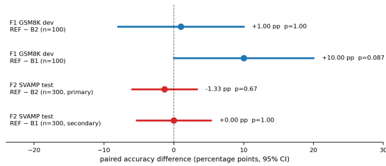
Figure 2: Paired accuracy differences with 95% bootstrap CIs (blue: F1 GSM8K dev; red: F2 locked SVAMP test). CIs are sampling uncertainty, not equivalence bounds: absence of a detectable difference does not establish that the compared configurations are equal.
