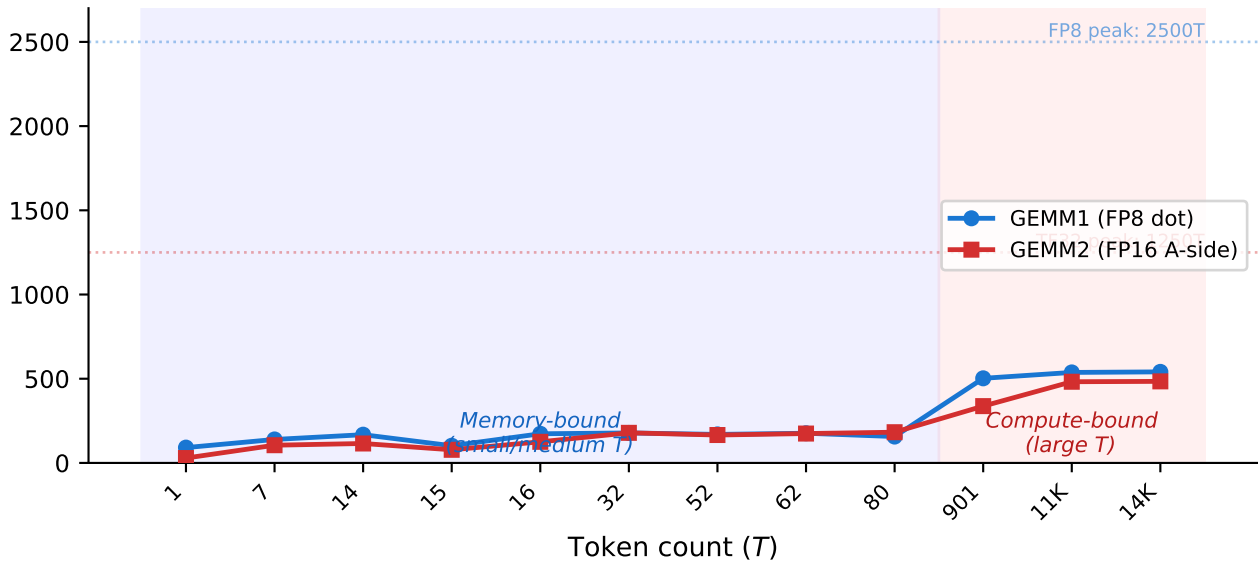
Effective TFLOPS
