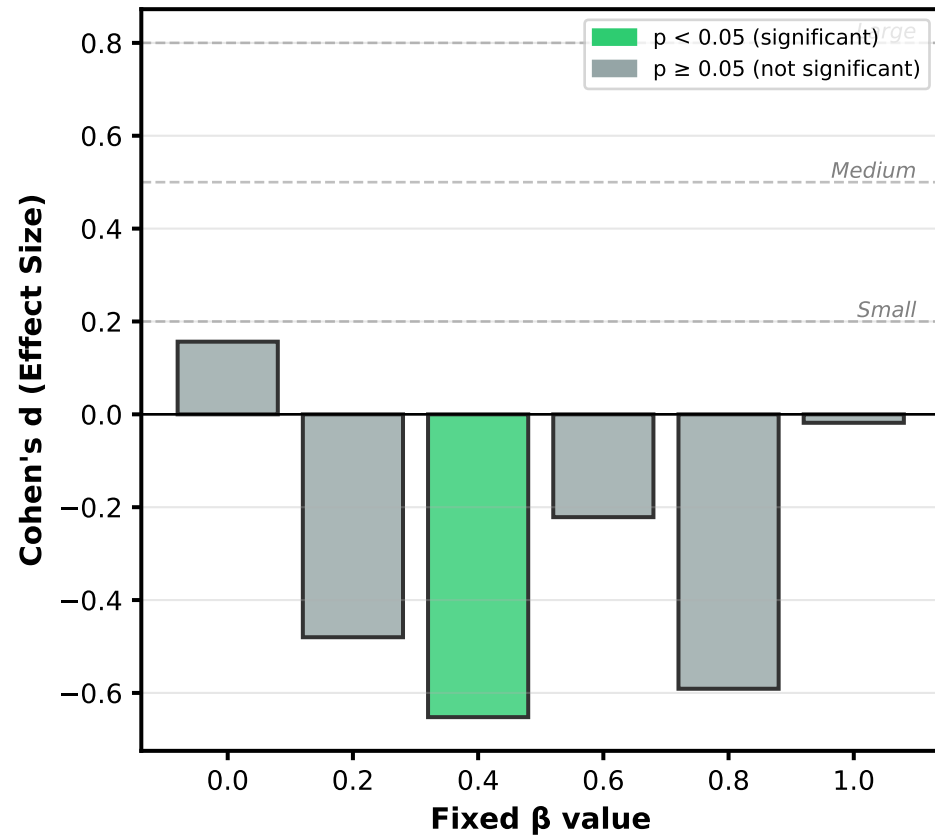
Volatility: 100 steps (Adaptive \beta vs Fixed \beta )
