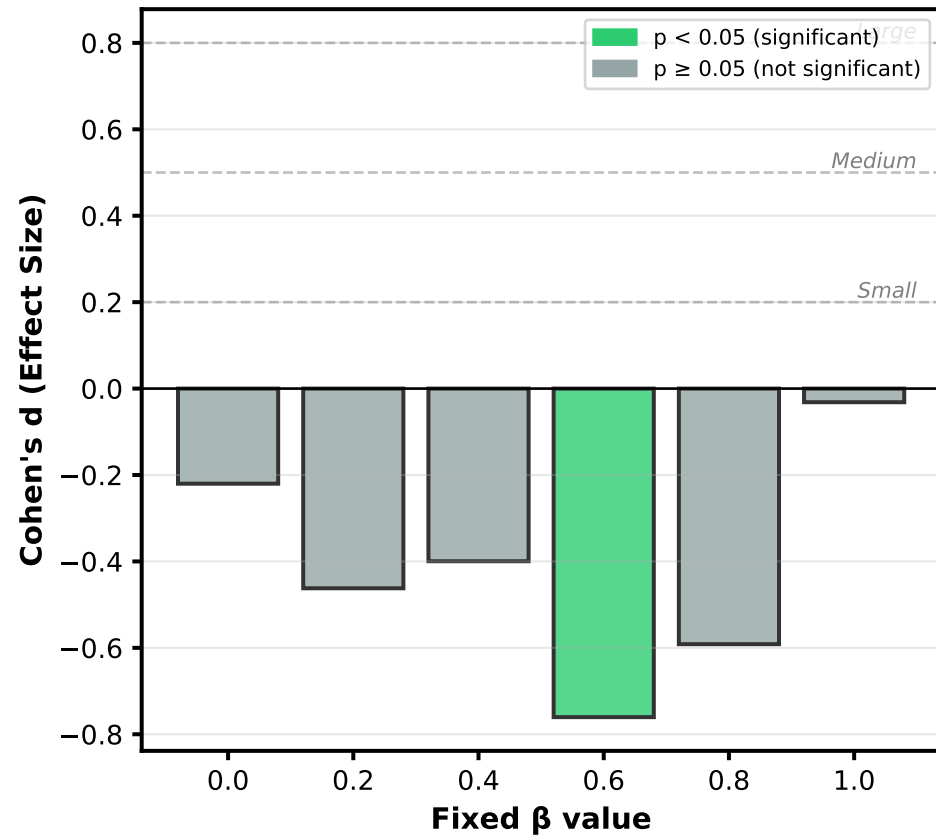
Volatility: 50 steps (Adaptive \beta vs Fixed \beta )
