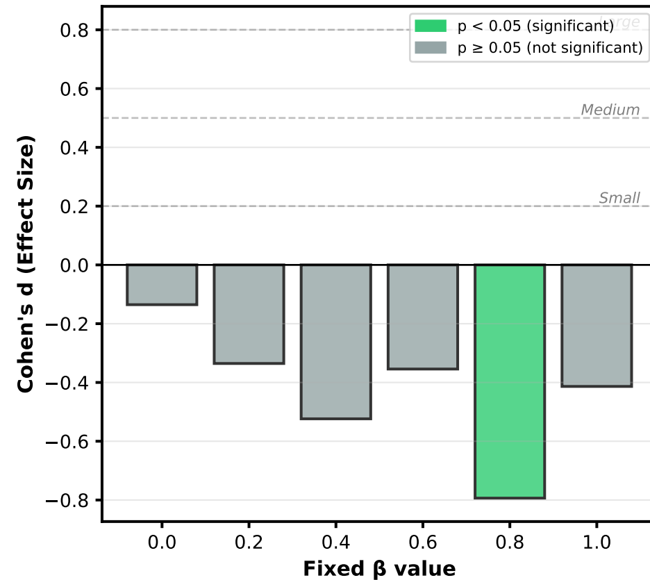
Volatility: 200 steps (Adaptive \beta vs Fixed \beta )
