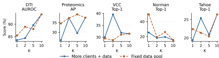
Figure 3: Effect of the number of laboratories. Solid lines add both laboratories and training data. Dashed lines divide the same training data across different numbers of laboratories. Full results are reported in Appendix B.
