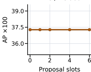
PTPC / heldout
