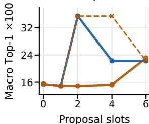
Norman / heldout
