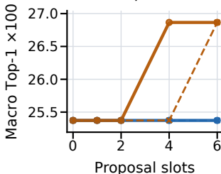
Tahoe / heldout
