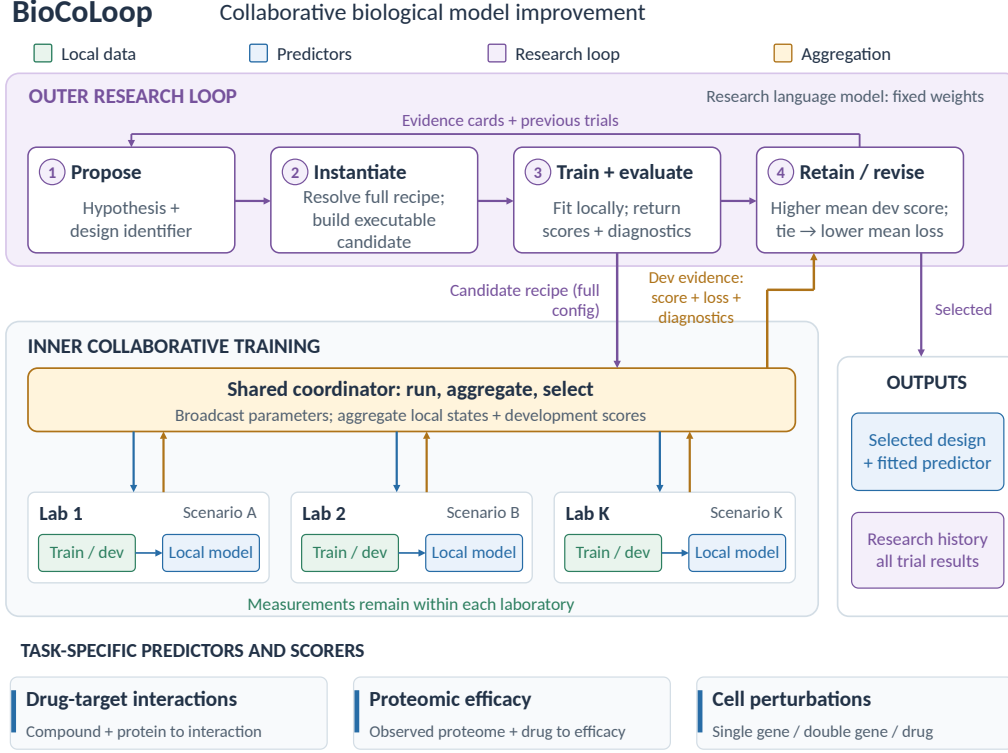
Figure 2: Data flow in BioCoLoop. The outer research loop proposes a complete candidate recipe and receives structured development evidence (scores, loss and bounded trajectory diagnostics) after its evaluation. The inner training process distributes model parameters to K laboratories, fits them locally and aggregates the returned states. The next proposal uses the accumulated research history. Task adapters implement drug–target interaction prediction, observed-response proteomic efficacy prediction and cell perturbation identification.
