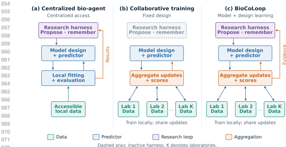
Figure 1: Research settings for biological AI. A centralized bio-agent revises a model using centrally accessible data; collaborative training lets K laboratories optimize a fixed recipe by sharing model updates; BioCoLoop additionally uses local evaluation to guide subsequent model and training changes.
