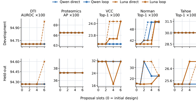
Figure 4: Research trajectories with and without evidence history in the six-slot protocol. Curves report development selection and held-out scores at each proposal prefix, where each candidate receives 100 rounds and slot 0 is the initial design.
