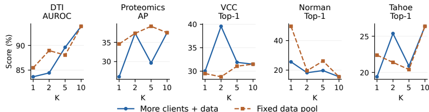
Figure 3: Effect of the number of laboratories. Solid lines add both laboratories and training data. Dashed lines divide the same training data across different numbers of laboratories. Full results are reported in Appendix B.
