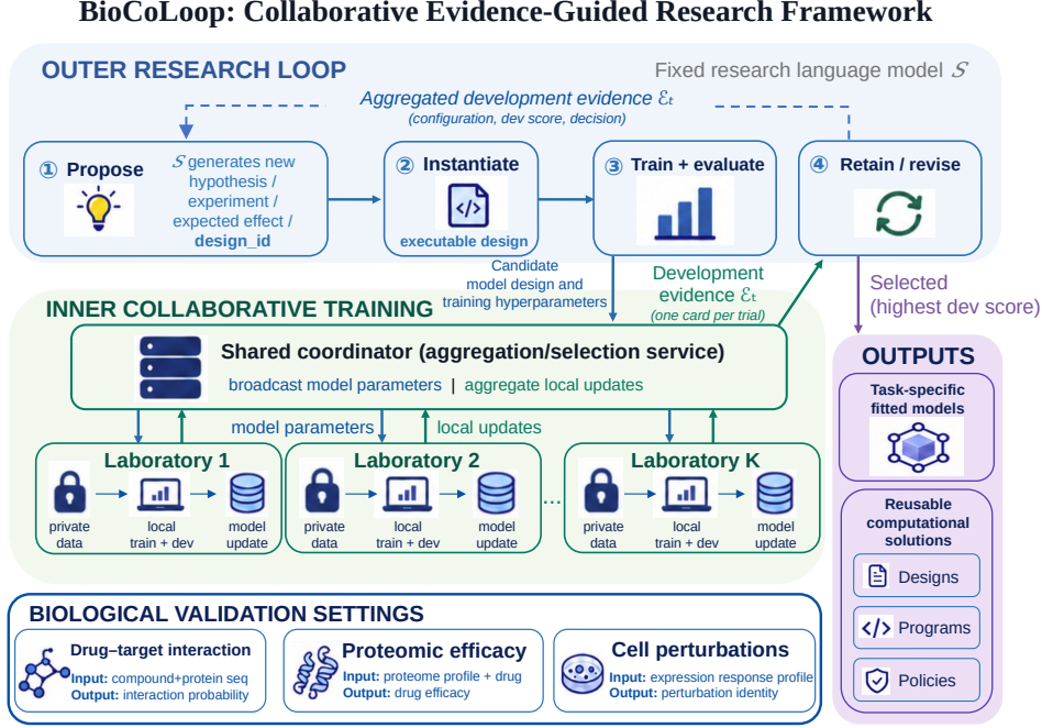
Figure 2: Data flow in BioCoLoop and the symbols used throughout. A candidate is an executable model configuration: a model design together with its training hyperparameters. The outer research loop is driven by the research model \mathcal{S} with fixed weights \theta , which proposes one candidate and receives the accumulated development evidence \mathcal{E}_t after each evaluation. Every trial appends one development-evidence card to the persistent set \mathcal{E}_t = \{e_1, \dots, e_t\} . A card records the executed configuration, the hypothesis, the best dev score and loss of the candidate and the acceptance decision. The shared coordinator of Section 3.1 is the logical service that resolves the candidate, distributes model parameters to K laboratories, fits them locally, aggregates the returned updates and summarizes each card. Section 3.2 defines the card and the dev score. The next proposal is conditioned on \mathcal{E}_t through Equation 3. Task adapters implement drug-target interaction prediction, observed-response proteomic efficacy prediction and cell perturbation identification.
