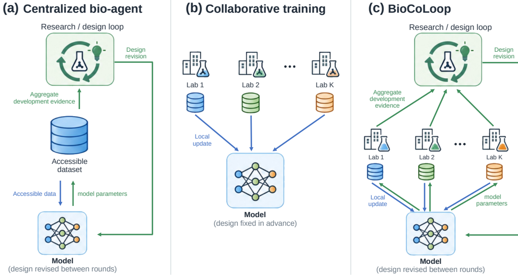
Figure 1: Research settings for biological AI. A centralized bio-agent revises a model using centrally accessible data. Collaborative training allows K laboratories to optimize the same model and training configuration by sharing model updates rather than raw data. BioCoLoop additionally uses results from local evaluation to guide subsequent changes to the model and training configuration.
