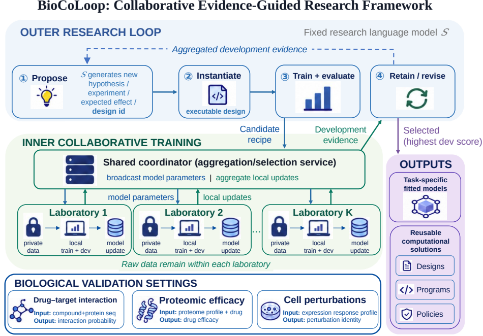
Figure 2: Data flow in BioCoLoop. The outer research loop proposes a model design and receives aggregate development evidence after its evaluation. The inner training process distributes model parameters to K laboratories, fits them locally and aggregates the returned updates. The next proposal uses the accumulated research history. Task adapters implement drug–target interaction prediction, observed-response proteomic efficacy prediction and cell perturbation identification.
