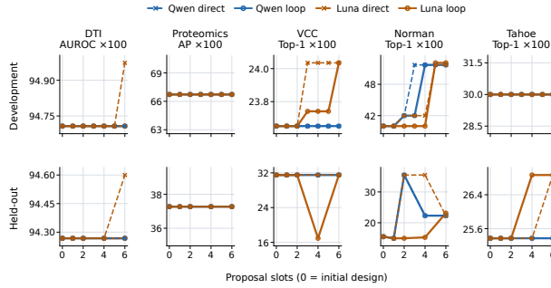
Figure 4: Research trajectories with and without evidence history. Curves report development selection and held-out scores at each proposal prefix; each candidate receives 100 rounds and slot 0 is the initial design.
