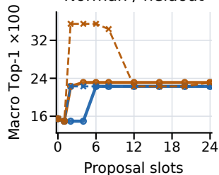
Norman / heldout
