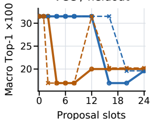
VCC / heldout
