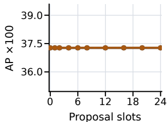
PTPC / heldout
