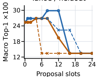
Tahoe / heldout
