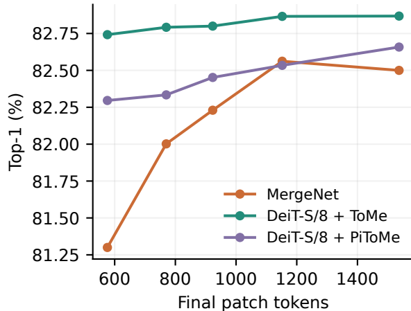
384 px, fine-tuned (MN R5.143)
