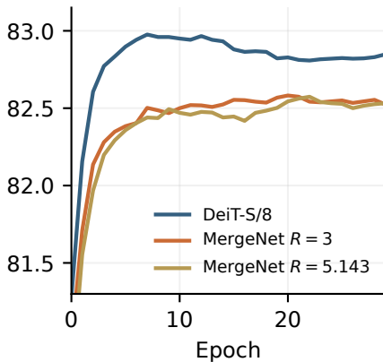
384 px fine-tune
