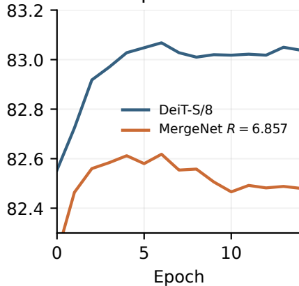
512 px fine-tune
