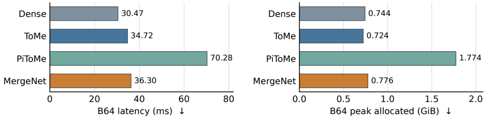
Figure 3: Batch-64 eager inference on the A100 with random weights. Bars show median latency and peak allocated memory from the same measurements as Table 5; lower is better.
