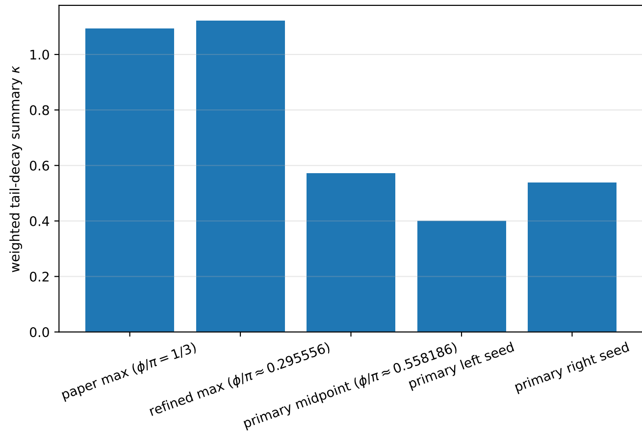
Weighted tail-decay summary at L = 300
