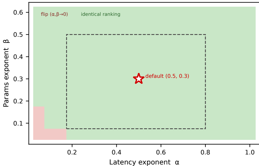
(a) LAE rank stability on the \alpha \times \beta grid
