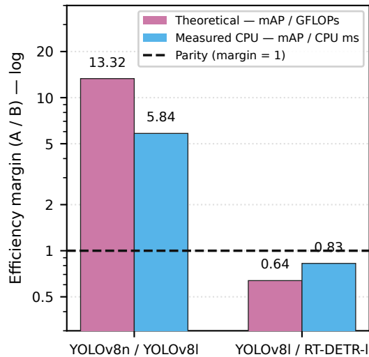
(b) FLOPs vs measured latency
