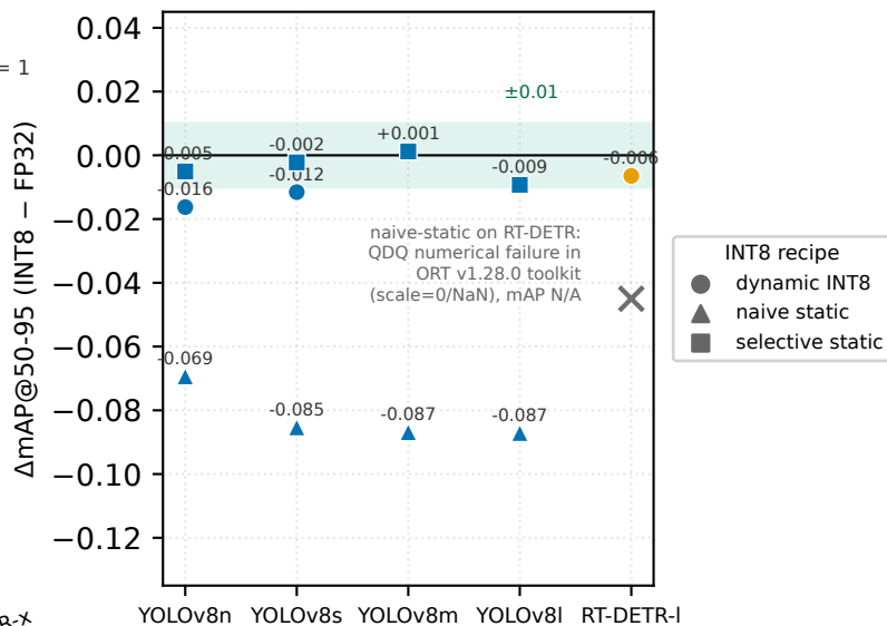
(b) Accuracy change, identical 500-image subset
