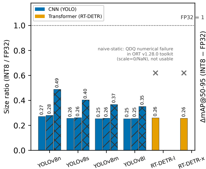
(a) Model size after INT8 (relative to FP32)
