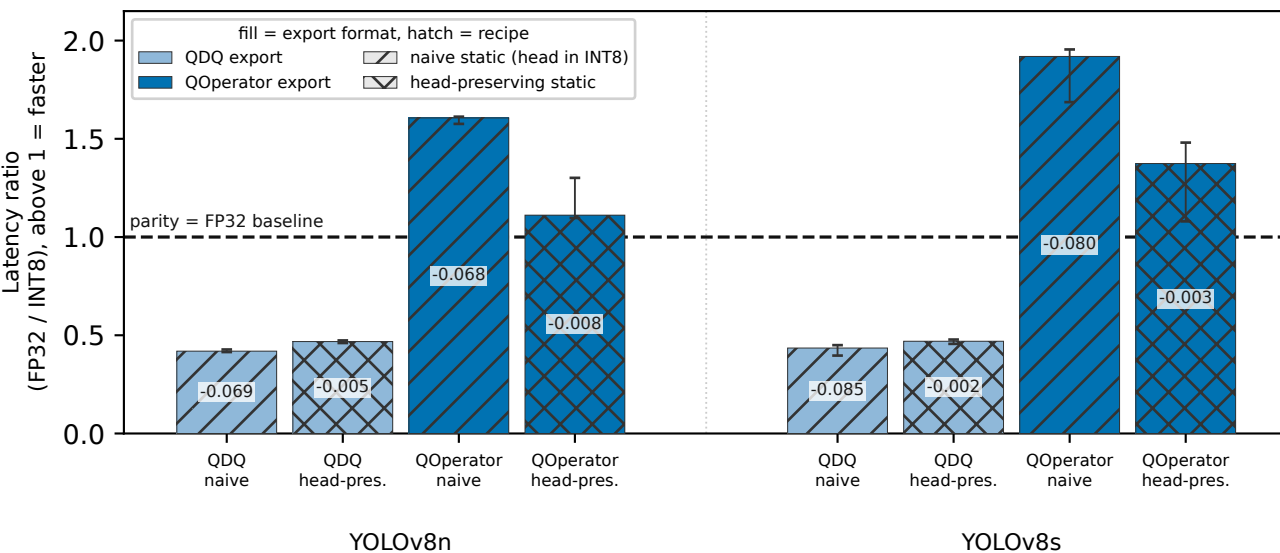
(c) Tested export paths show different INT8 latency
