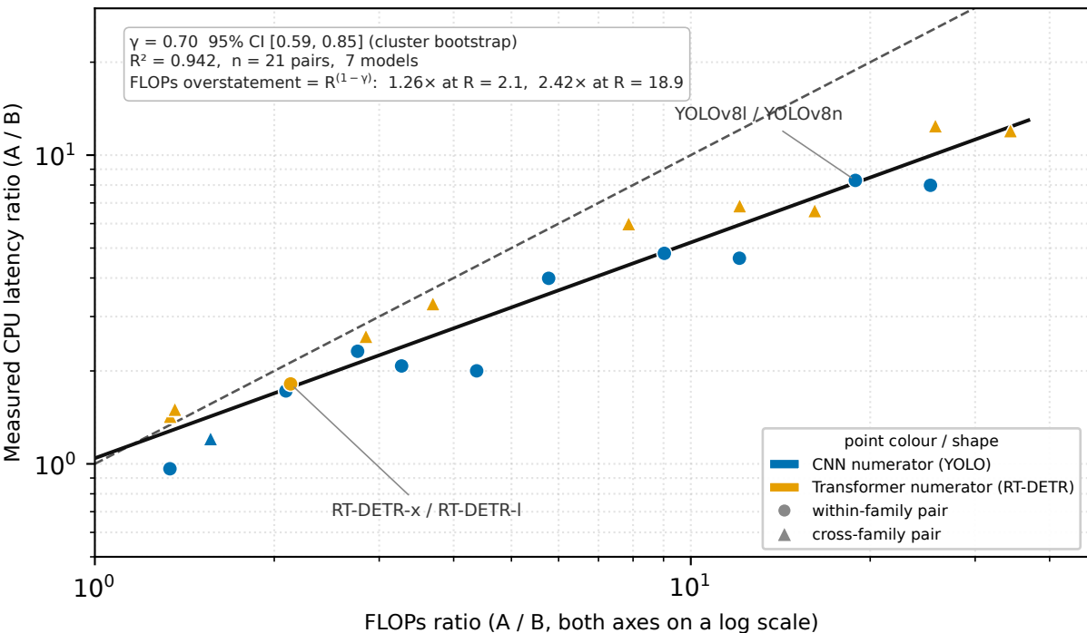
FLOPs-to-latency scaling across all 21 model pairs
