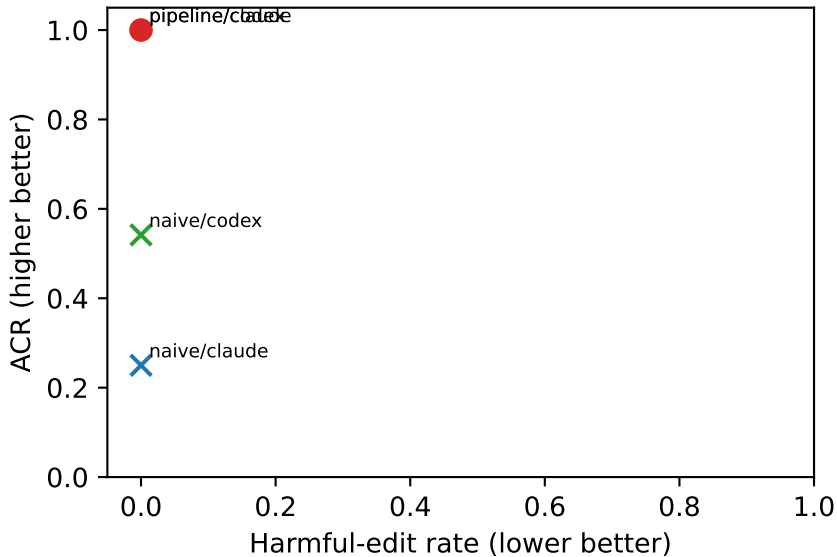
Recall vs harmful-edit frontier
