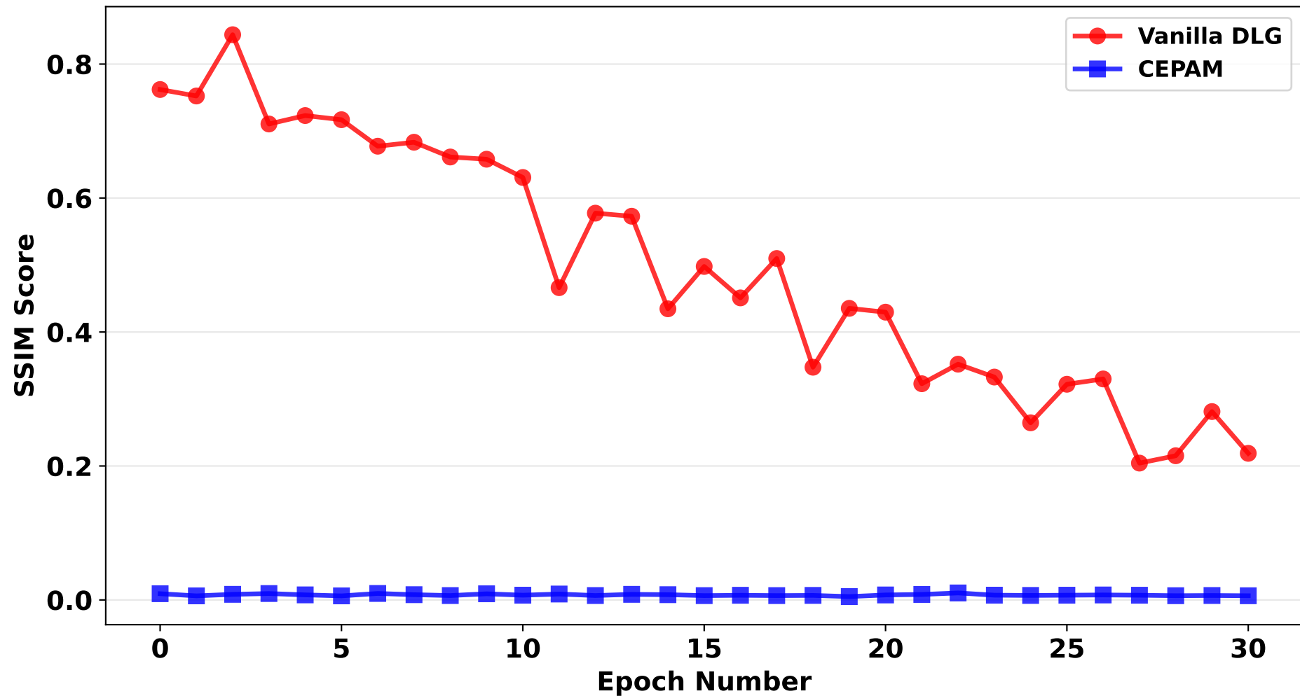
SSIM Score of Vanilla DLG and CEPAM vs Epoch Number ( n=1 , b=0.005 )
