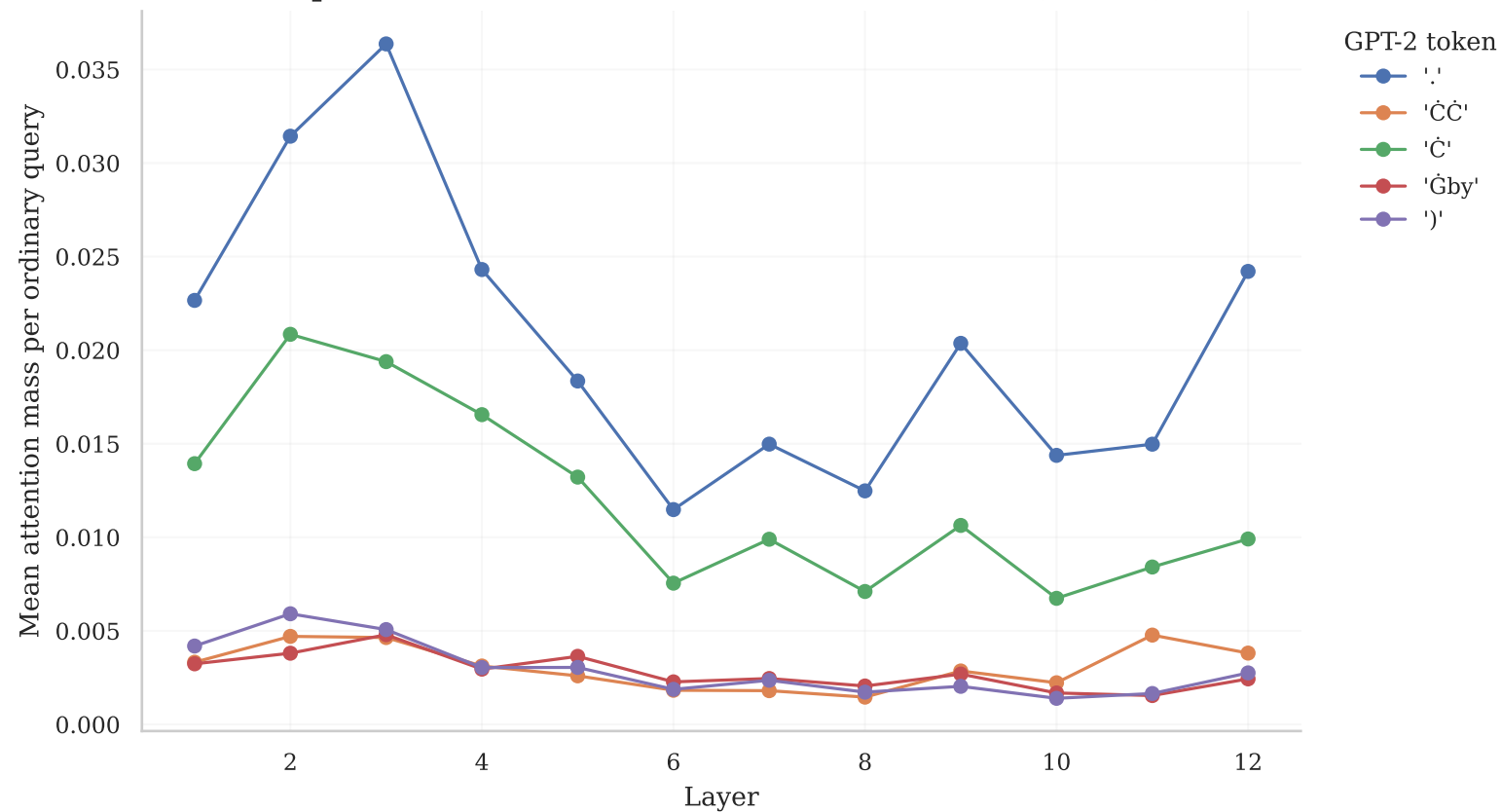
Top attention-sink candidates for GPT-2 Heads (N=158)
