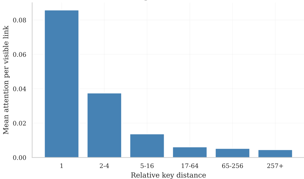
Distance baseline diagnostic for GPT-2 heads (N=158)
