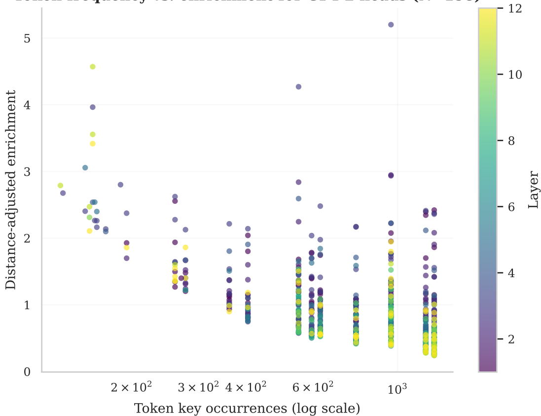
Token frequency vs. enrichment for GPT-2 heads (N=158)
