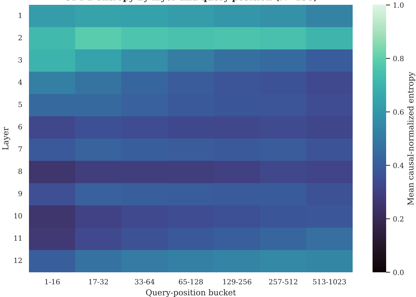
GPT-2 entropy by layer and query position (N=158)
