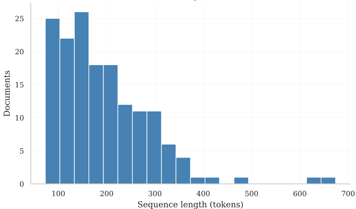
GPT-2 attention-shard length distribution (N=158)
